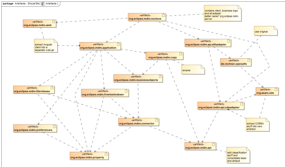
Figure 1 Dependency Graph (Should Be)
